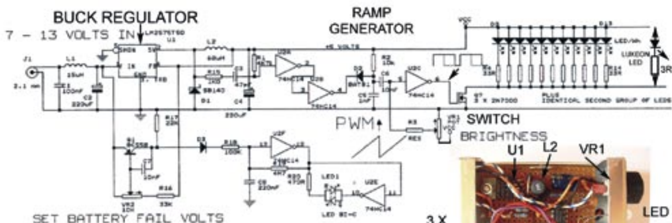
Fig. 5 CIRCUIT DIAGRAM
