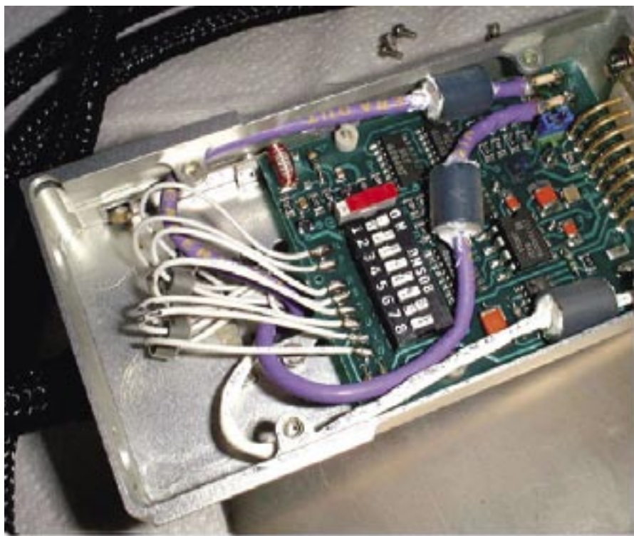
An enlargement of the Ikegami HL79D camera interface module type NV-ICP-AG.
