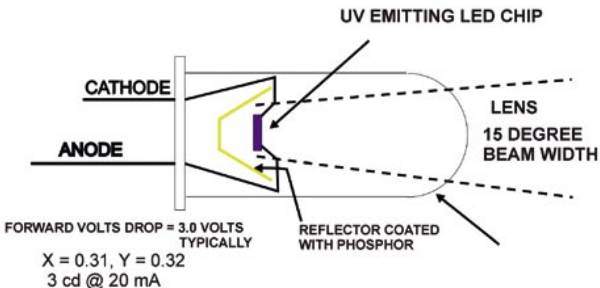
FIG. 1 WHITE LED X-OPTO WT5111A
